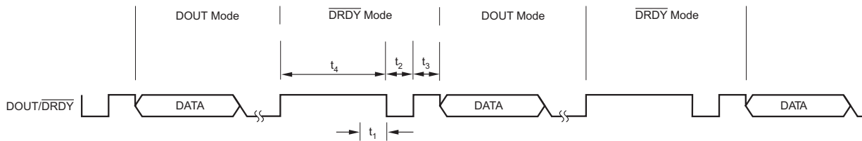
Figure 31. DOUT/DRDY Partitioning
