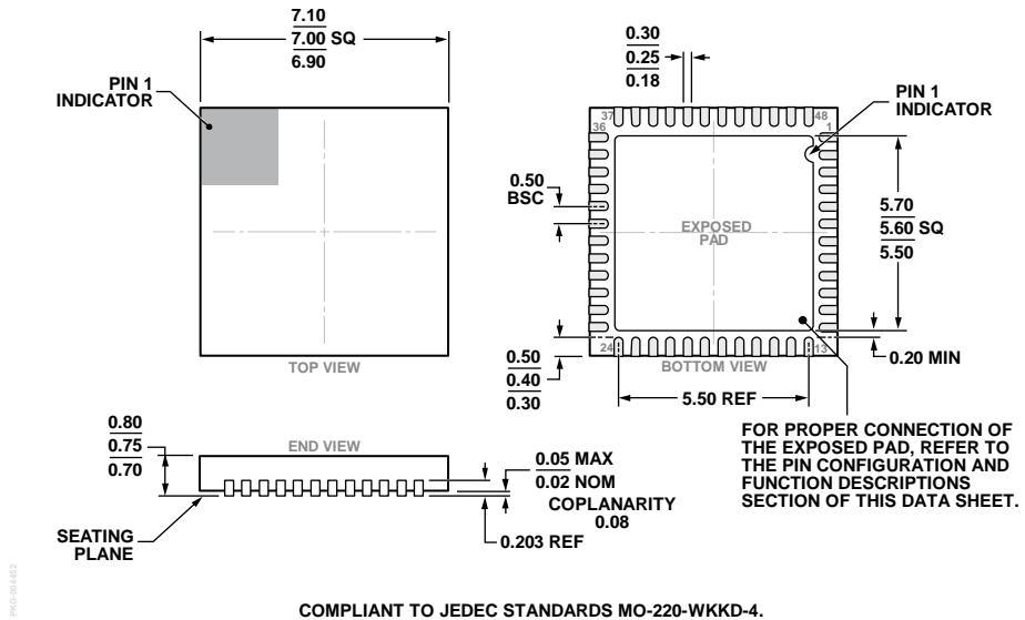
Figure 107. 48-Lead Lead Frame Chip Scale Package [LFCSP] 7 mm × 7 mm Body and 0.75 mm Package Height (CP-48-13) Dimensions shown in millimeters
