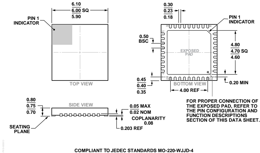
Figure 44. 36-Lead Lead Frame Chip Scale Package [LFCSP] 6 mm × 6 mm Body and 0.75 mm Package Height (CP-36-5)
