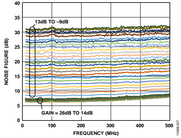
Figure 27. Noise Figure vs. Frequency for 35 dB Gain Range at V_{POS} = 3.3 V , Low Power Mode
