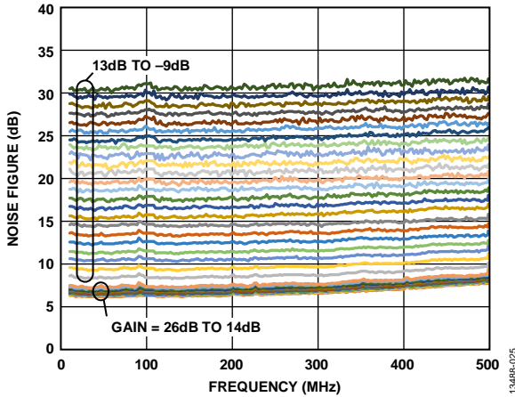
Figure 25. Noise Figure vs. Frequency for 35 dB Gain Range at V_{POS} = 3.3 V , High Performance Mode
