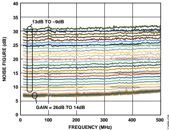
Figure 26. Noise Figure vs. Frequency for 35 dB Gain Range at V_{POS} = 5 V , Low Power Mode
