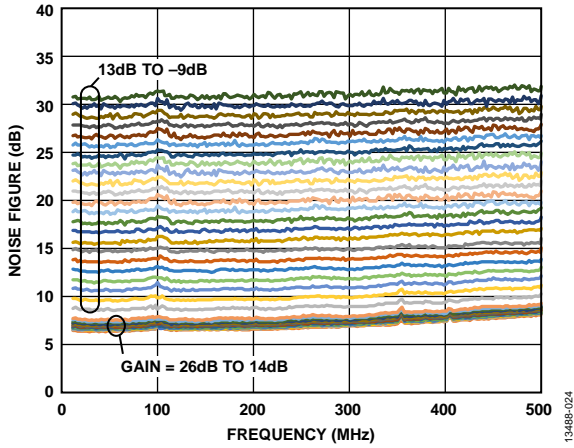
Figure 24. Noise Figure vs. Frequency for 35 dB Gain Range at V_{POS} = 5 V , High Performance Mode
