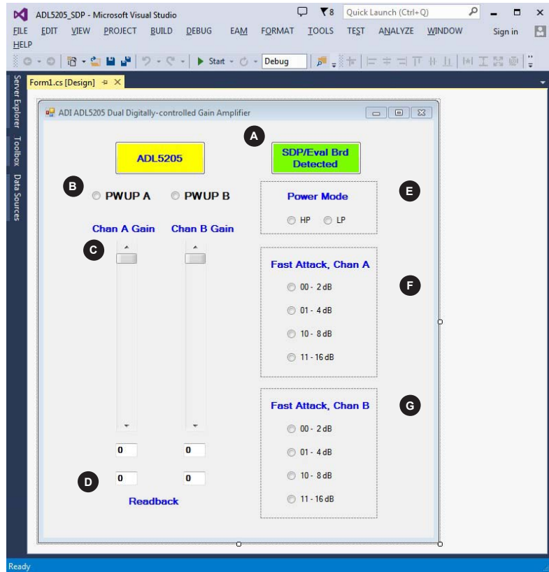
Figure 65. Main Screen of the ADL5205 Control Software
