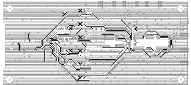
Figure 63. Bottom Layer
