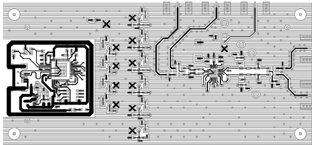
Figure 62. Top Layer
