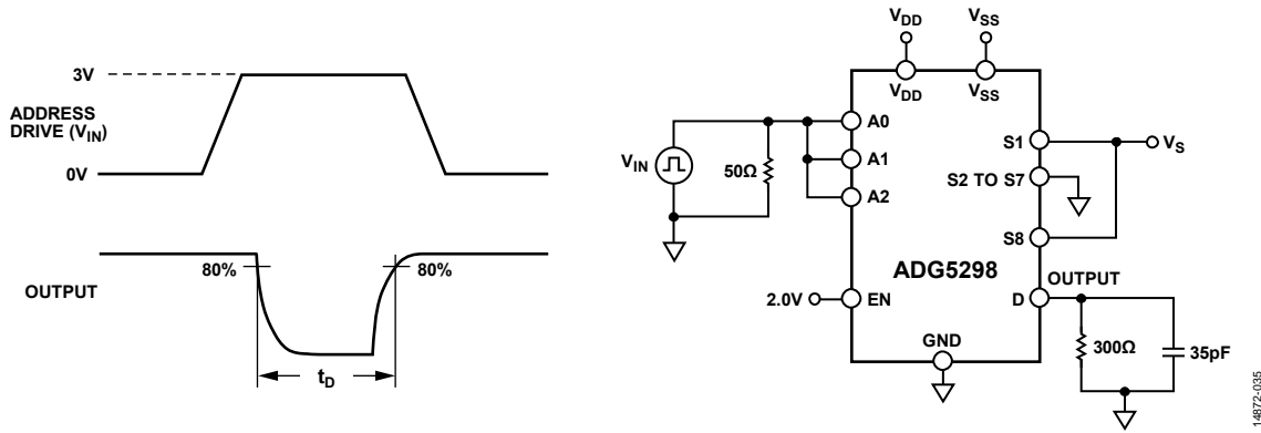
Figure 37. Break-Before-Make Time Delay, t_b
