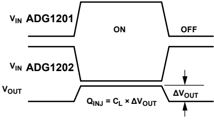
Figure 27. Charge Injection
