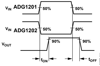
Figure 26. Switching Times
