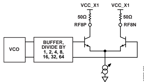
Figure 41. Output Stage
