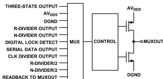
Figure 19. MUXOUT Schematic
