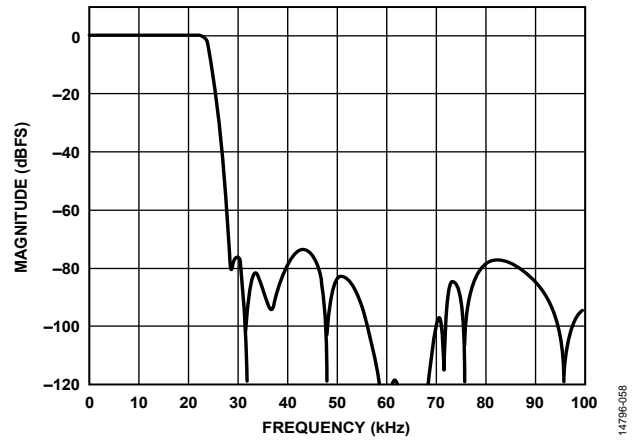
Figure 50. Total Interpolation Response, f_s = 768 kHz
