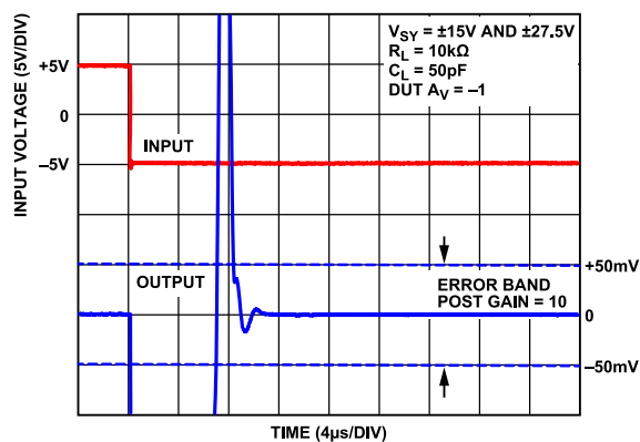
Figure 70. Positive Settling Time to 0.1%, V_{SY} = \pm 15\text{ V} and \pm 27.5\text{ V}
