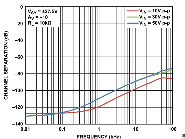
Figure 47. Channel Separation vs. Frequency, V_{SY} = \pm 27.5 V
