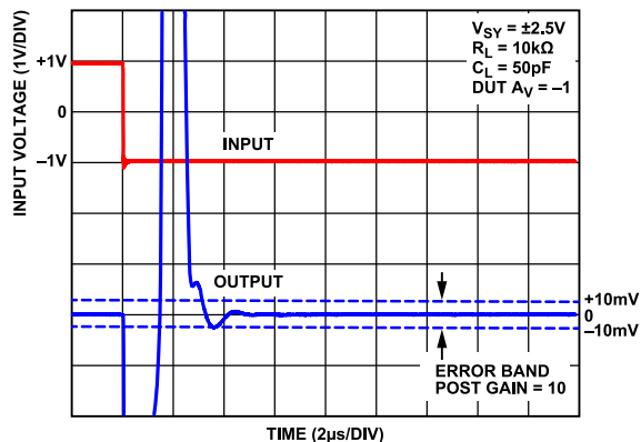
Figure 66. Negative Settling Time to 0.1%, V_{SY} = \pm 2.5\text{ V}
