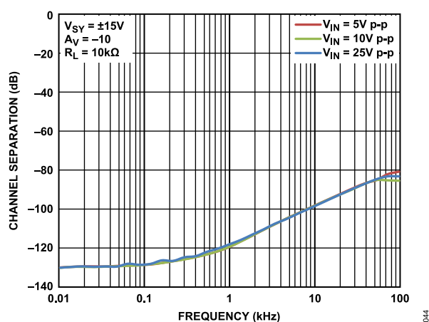
Figure 46. Channel Separation vs. Frequency, V_{SY} = \pm 15 V
