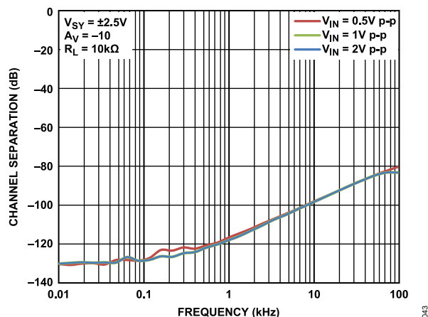
Figure 45. Channel Separation vs. Frequency, V_{SY} = \pm 2.5 V
