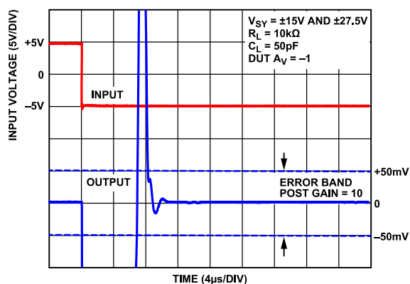
Figure 67. Negative Settling Time to 0.1%, V_{SY} = \pm 15\text{ V} and \pm 27.5\text{ V}
