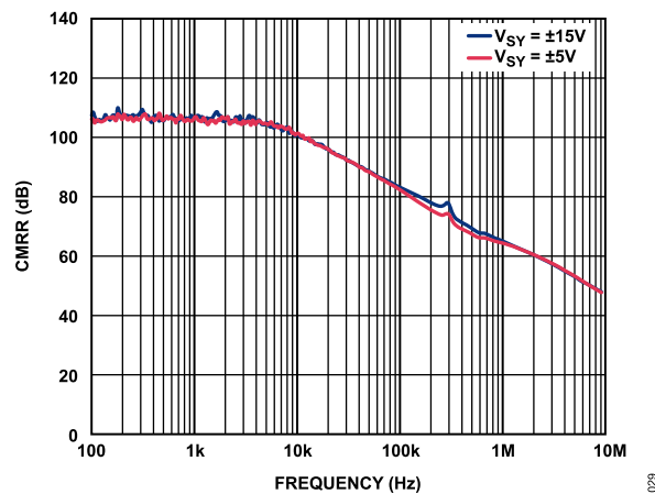
Figure 37. CMRR vs. Frequency, V_{SY} = \pm 5\text{ V and } V_{SY} = \pm 15\text{ V}
