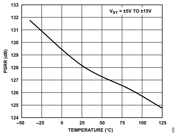
Figure 34. PSRR vs. Temperature, V_{SY} = \pm 5\text{ V to } \pm 15\text{ V}
