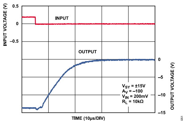
Figure 51. Negative Overload Recovery, V_{SY} = \pm 15\text{ V}
