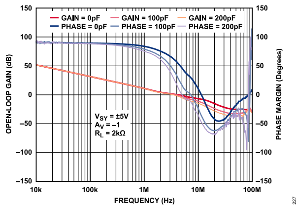
Figure 30. Open-Loop Gain and Phase Margin vs. Frequency, V_{SY} = \pm 5\text{ V}
