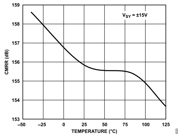
Figure 39. CMRR vs. Temperature, V_{SY} = \pm 15\text{ V}
