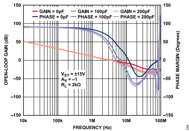
Figure 33. Open-Loop Gain and Phase Margin vs. Frequency, V_{SY} = \pm 15\text{ V}
