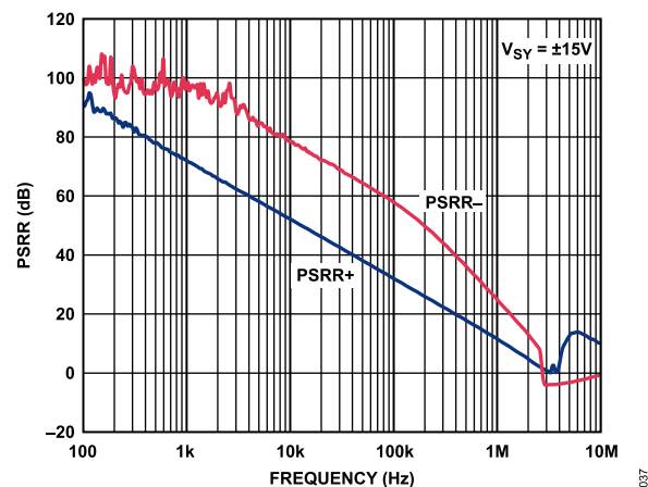
Figure 38. PSRR vs. Frequency, V_{SY} = \pm 15\text{ V}
