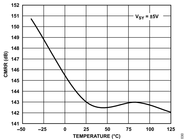
Figure 36. CMRR vs. Temperature, V_{SY} = \pm 5\text{ V}
