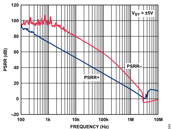
Figure 35. PSRR vs. Frequency, V_{SY} = \pm 5\text{ V}
