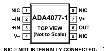
Figure 1. ADA4077-1, 8-Lead SOIC and 8-Lead MSOP
