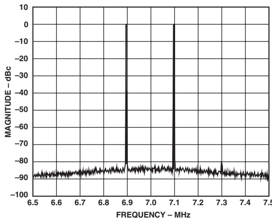
TPC 12. Dual-Tone Spectral Plot @ f_{DATA} = 50\text{ MSPS} , f_{OUT} = 6.9\text{ MHz} and 7.1\text{ MHz} , 2\times\text{ LPF}
