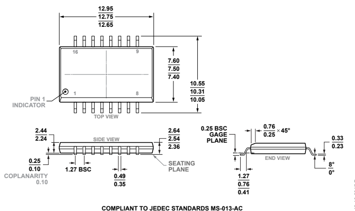
Figure 37. 16-Lead Standard Small Outline Package, with Increased Creepage [SOIC_IC] Wide Body (RI-16-2) Dimensions shown in millimeters
