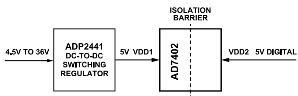
Figure 36. ADP2441 Step-Down DC-to-DC Regulator Example
