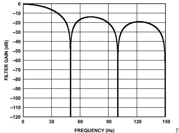
Figure 101. 50 Hz Rejection
