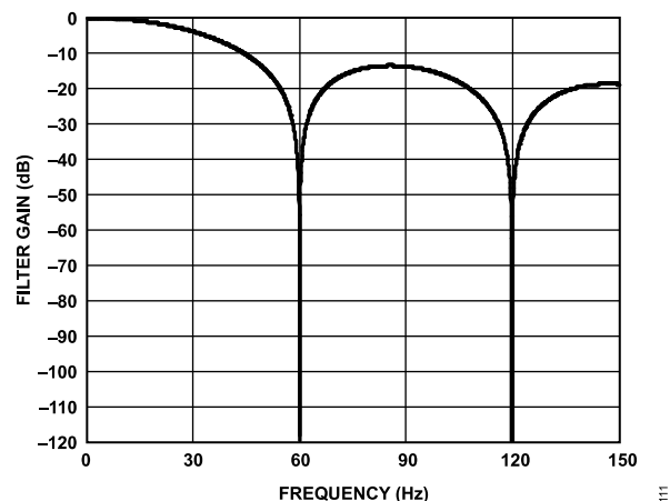
Figure 102. 60 Hz Rejection
