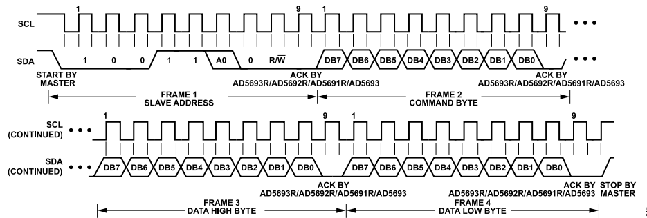
Figure 47. I 2 C Write Operation
