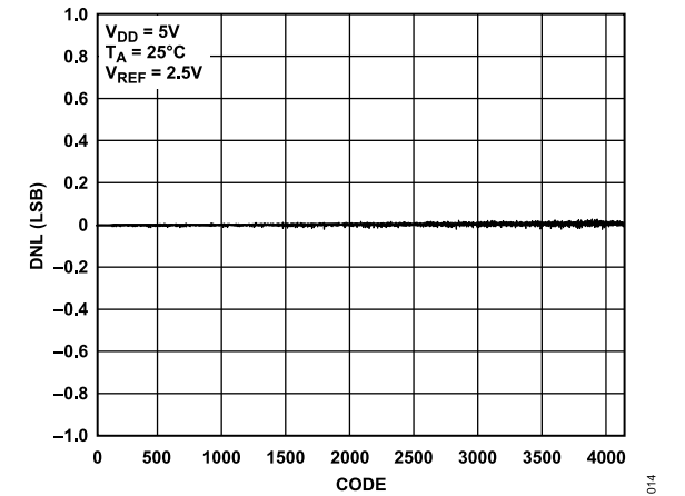
Figure 14. AD5691R DNL
