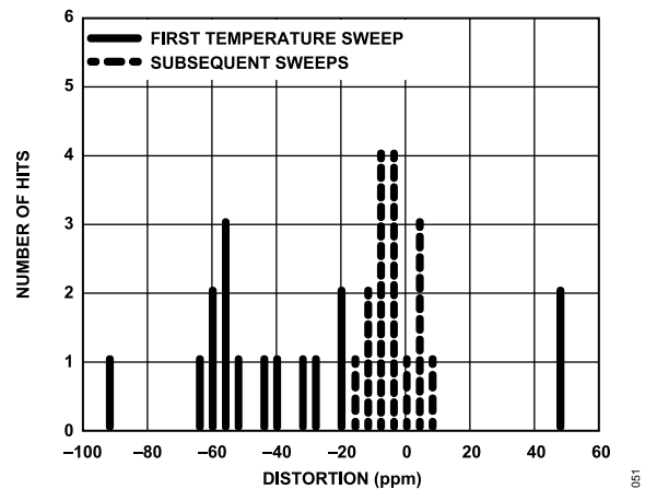
Figure 50. Thermal Hysteresis
