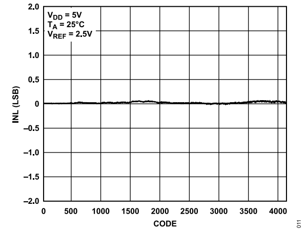
Figure 11. AD5691R INL
