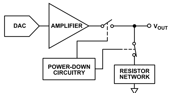
Figure 48. Output Stage During Power-Down
