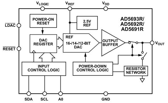
Figure 1. MSOP
