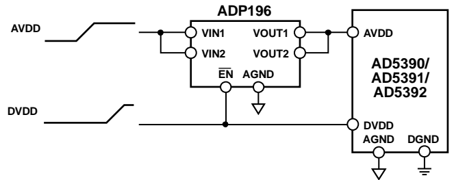
Figure 43. AV DD Power Supply Controlled by a Load Switch
