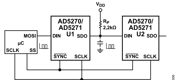
Figure 44. Daisy-Chain Configuration Using SDO
