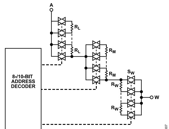
Figure 45. Simplified RDAC Circuit
