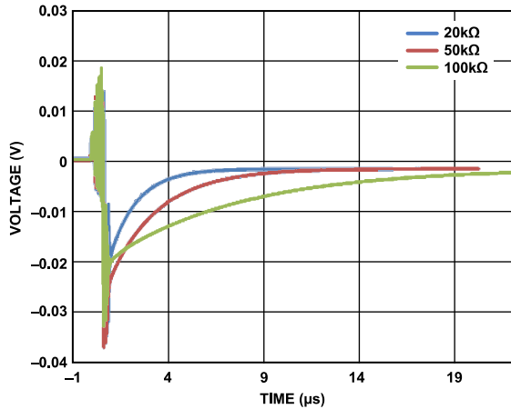
Figure 33. Maximum Glitch Energy
