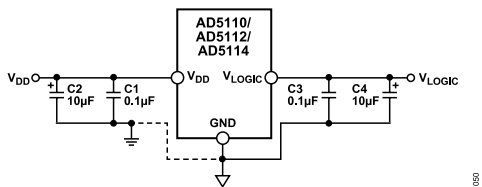
Figure 50. Power Supply Bypassing
