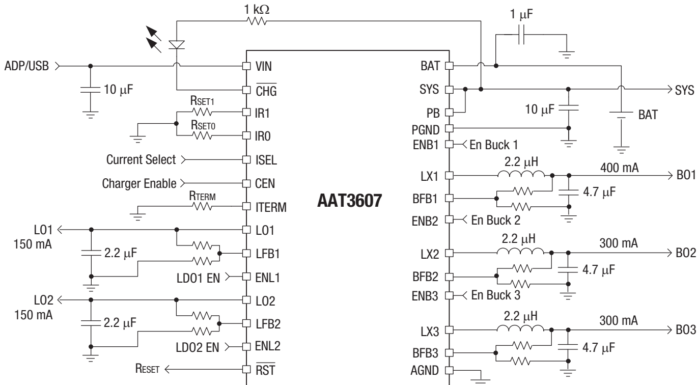
Figure 1. AAT3607 Typical Application Circuit
