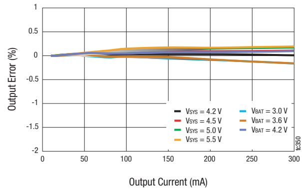
Figure 12. Buck 3 DC Regulation ( V_{out} = 1.2\text{ V} , L = 2.2\ \mu\text{H} )
