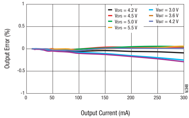
Figure 10. Buck 2 DC Regulation ( V_{out} = 1.8\text{ V} , L = 2.2\ \mu\text{H} )
