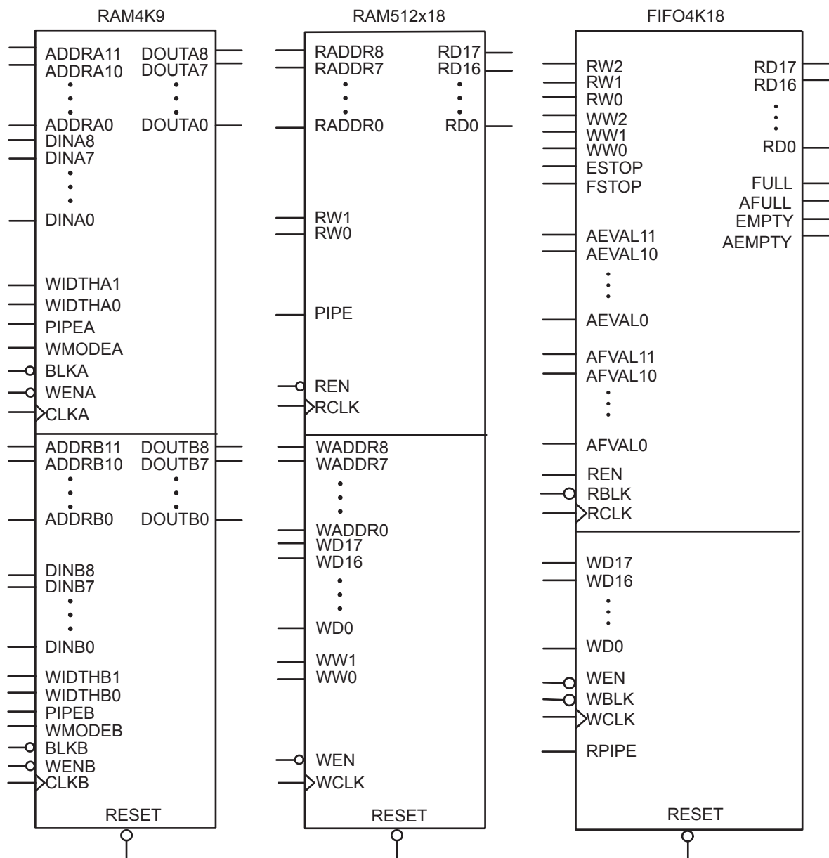
Figure 2-30 • RAM Models
