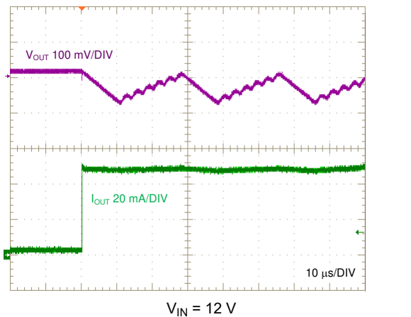
Figure 8-19. Load Transient, 0 mA to 50 mA, 1 A/μs
