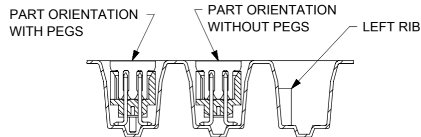
SECTION Z-Z
