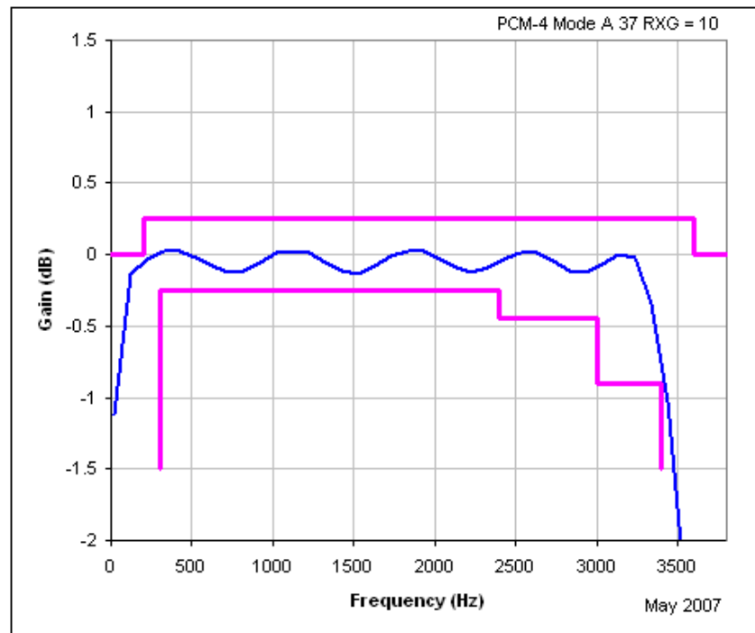
Figure 44: Gain versus Frequency for Analog Input at the Line to the Digital DX Output
