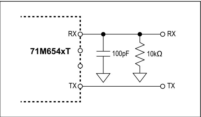
Figure 14. Typical UART Operating Circuit
