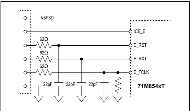
Figure 16. Typical Emulator Connections
