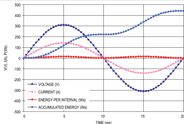
Figure 6. Waveforms Comparing Voltage, Current, Energy per Interval, and Accumulated Energy
