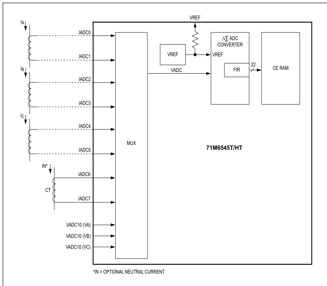
Figure 2. 71M6545T/HT Operating with Local Sensors
