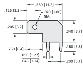
.205 (5.2) TAB
