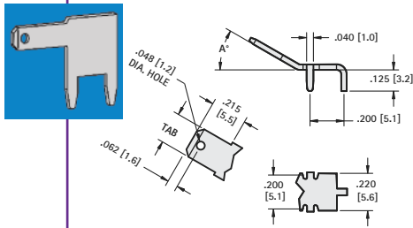
.110 (2.8) & .187 (4.8) TAB
