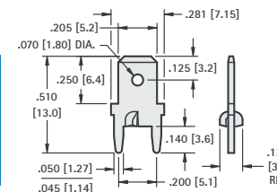
.205 (5.2) TAB
