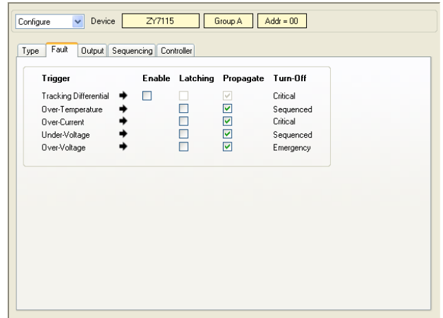
Figure 40. Fault Management Window
