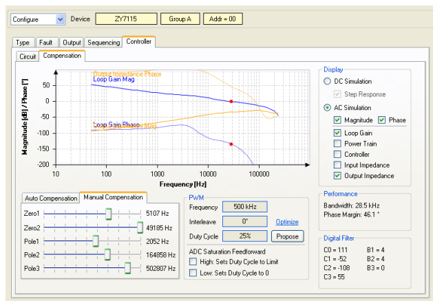
Figure 47. PWM Controller Window
