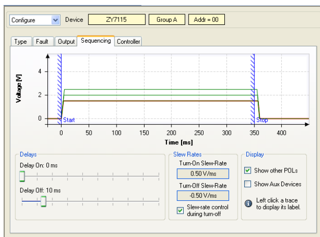
Figure 32. Sequencing/Tracking Window
