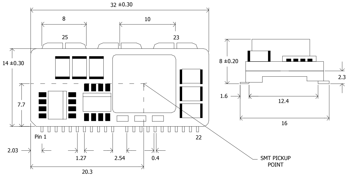
Figure 57. Mechanical Drawing
