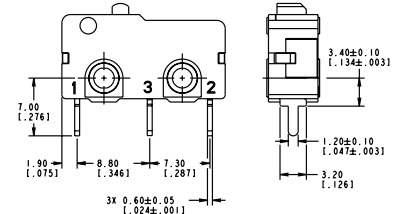
Terminal Type 20 - Straight PCB
