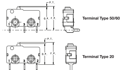
Operate Point References for PCB Terminals
