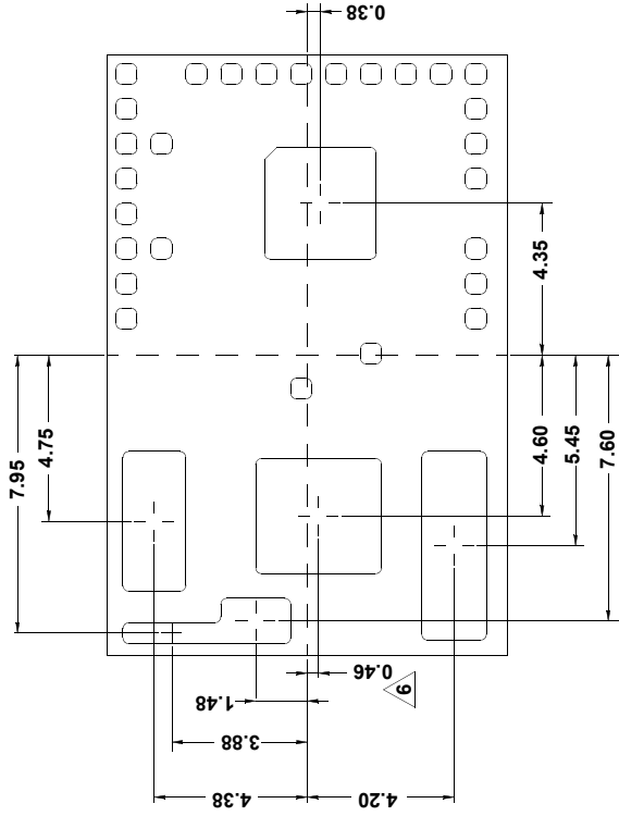
CENTERLINE POSITION DETAILS FOR THE 5 EXPOSED DAPS BOTTOM VIEW
