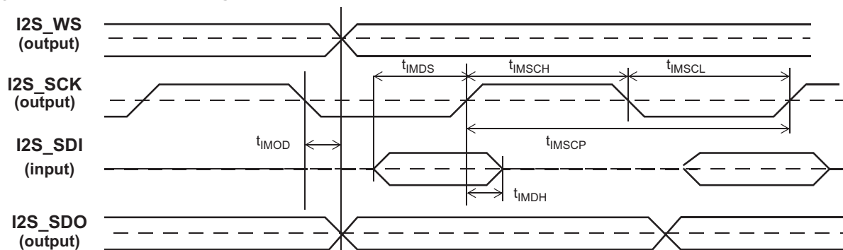
Figure 38 • Master I 2 S Timing
