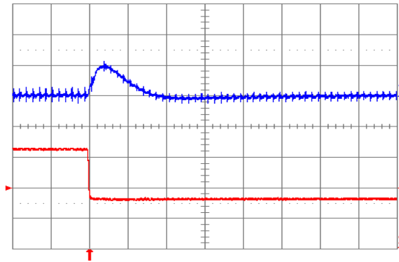
Fig. 1.5V.7: Output voltage response for V_{out} = 1.5\text{ V} to negative load current step change from 16 A to 8 A with slew rate of -5 A/μs at V_{in} = 12\text{ V} . Top trace: output voltage (200 mV/div.); Bottom trace: load current (5 A/div.). C_o = 100\text{ μF} ceramic. Time scale: 20 μs/div.
