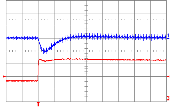
Fig. 1.5V.6: Output voltage response for V_{out} = 1.5\text{ V} to positive load current step change from 8 A to 16 A with slew rate of 5 A/μs at V_{in} = 12\text{ V} . Top trace: output voltage (200 mV/div.); Bottom trace: load current (5 A/div.). C_o = 100\text{ μF} ceramic. Time scale: 20 μs/div.
