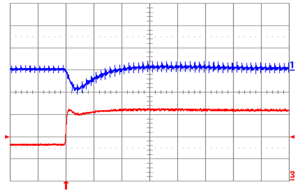
Fig. 1.0V.6: Output voltage response for V_{out} = 1.0 V to positive load current step change from 8 A to 16 A with slew rate of 5 A/ \mu\text{s} at V_{in} = 12 V. Top trace: output voltage (200 mV/div.); Bottom trace: load current (5 A/div.). C_o = 100 \mu\text{F} ceramic. Time scale: 20 \mu\text{s} /div.
