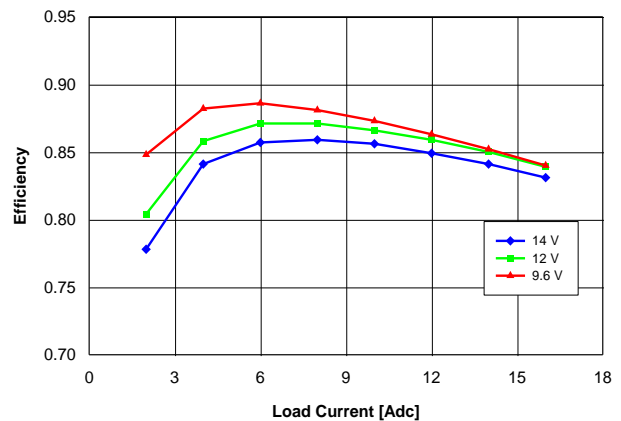
Fig. 1.2V.2: Efficiency vs. load current and input voltage for V_{out} = 1.2\text{ V} converter mounted vertically with air flowing at a rate of 200 LFM (1 m/s) and T_a = 25\text{ °C} .
