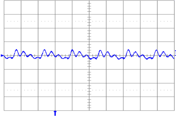
Fig. 1.5V.5: Output voltage ripple (20 mV/div.) at full rated load current into a resistive load with external capacitance 100 μF ceramic + 1 μF ceramic and V_{in} = 12\text{ V} for V_{out} = 1.5\text{ V} . Time scale: 2 μs/div.
