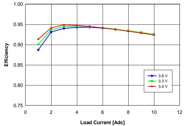
Fig. 2.0V.4: Efficiency vs. load current and input voltage for V_{out} = 2.0\text{ V} converter mounted horizontally with air flowing at a rate of 200 LFM (1 m/s) and T_a = 25\text{ }^{\circ}\text{C} .
