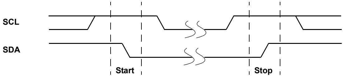
Figure 2. Valid Start and Stop Conditions
