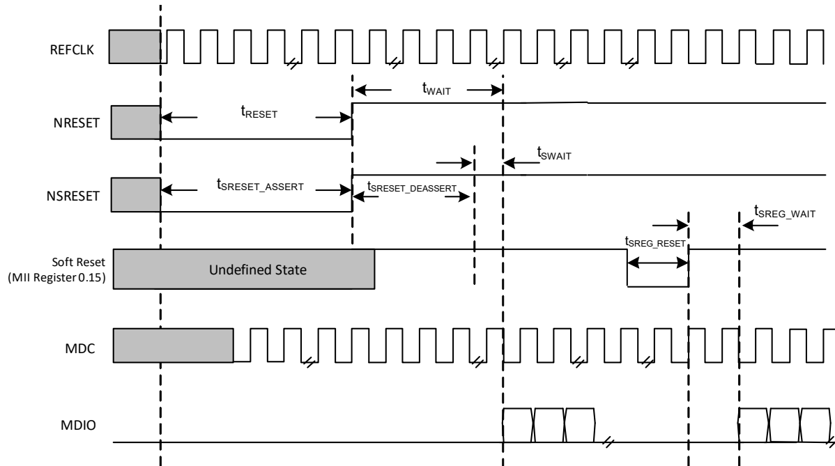
Figure 21 • Reset Timing
