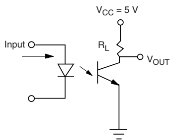
Fig. 2 - Test Circuit
