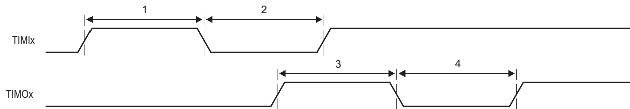
Figure 7-62 Timer Timing
