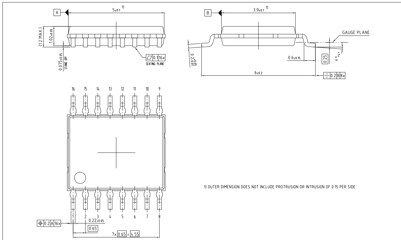
Figure 23 Package dimensions
