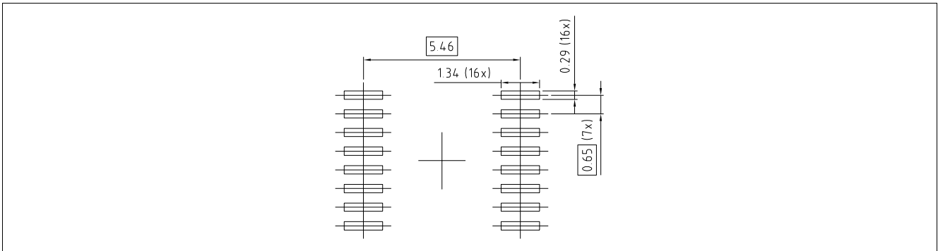
Figure 26 Footprint
