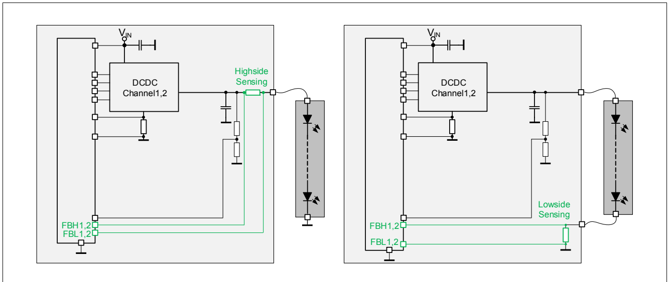
Figure 10 Highside and lowside current sensing - TLD5541-2QV
