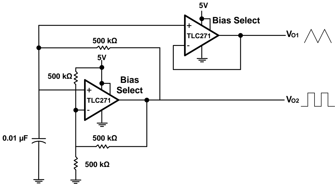
Figure 110 Multivibrator
