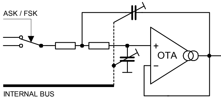
Figure 7 Data Filter Architecture
