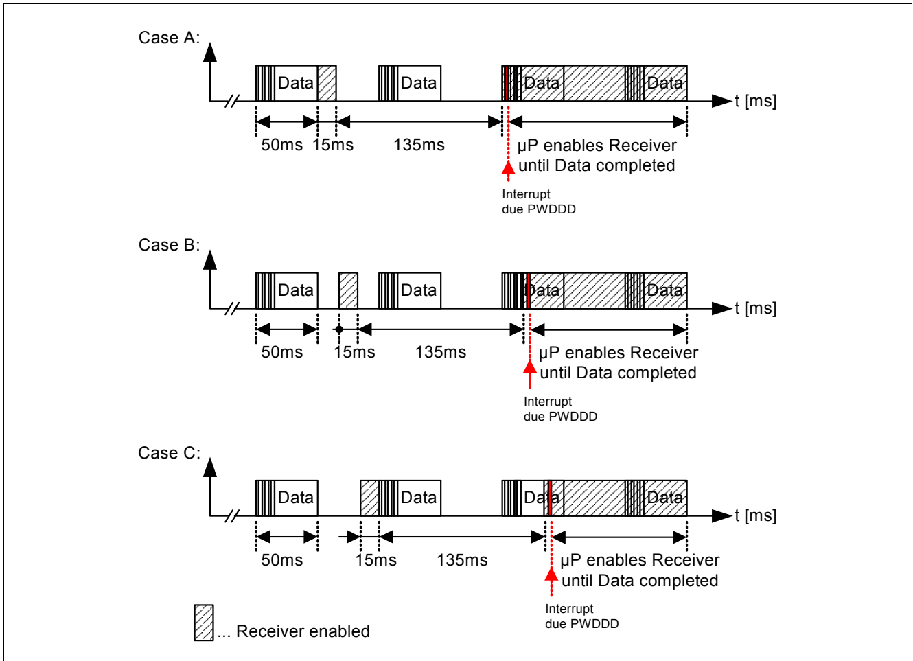
Figure 53 3 Possible Timings
