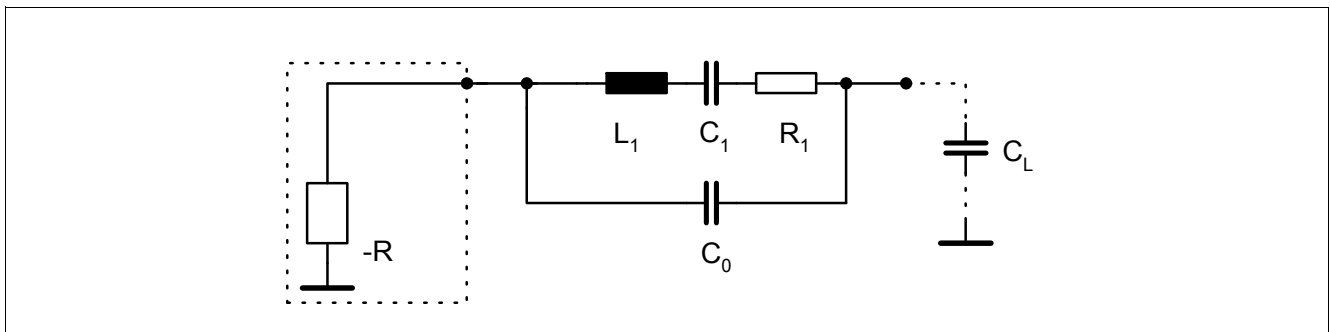
Figure 32 Crystal
