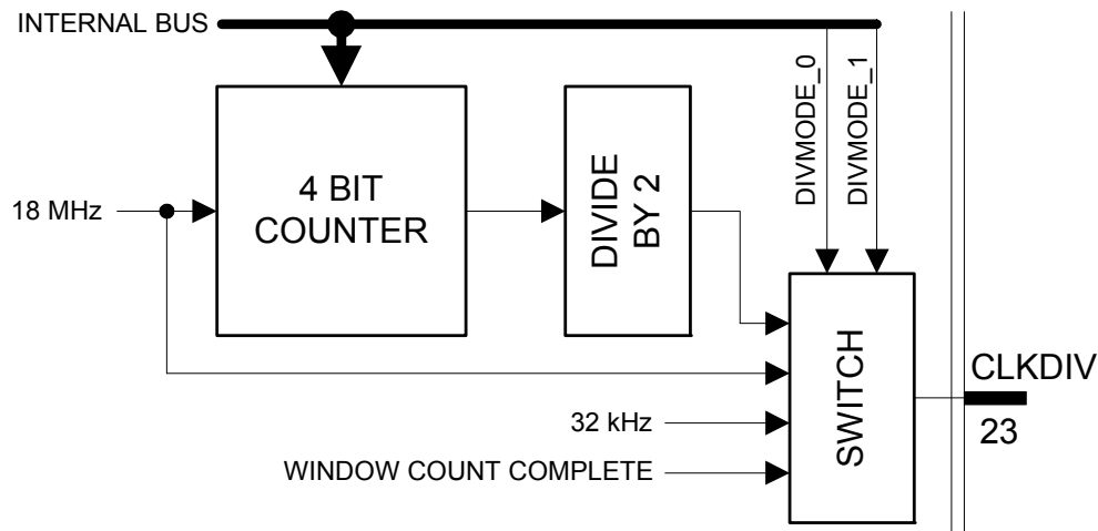
Figure 20 Clock Divider
