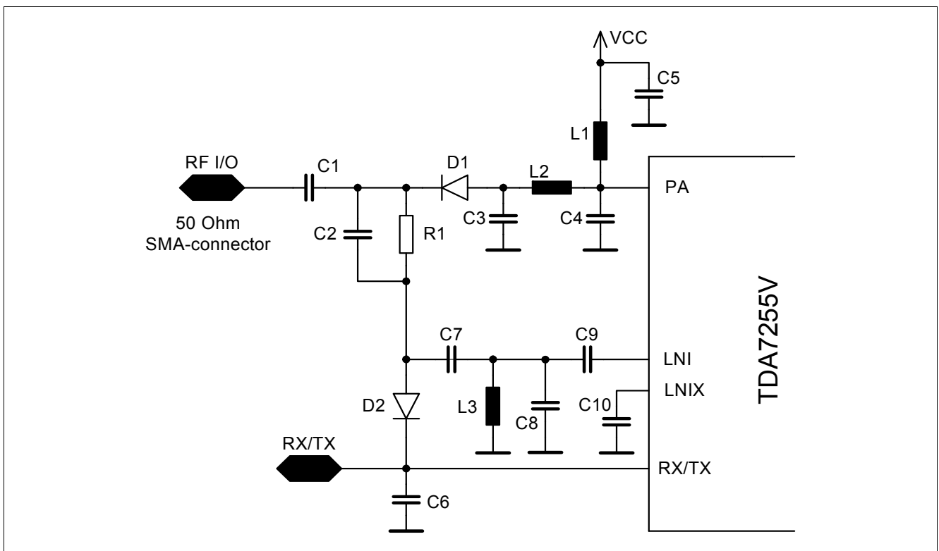
Figure 21 RX/TX-Switch
