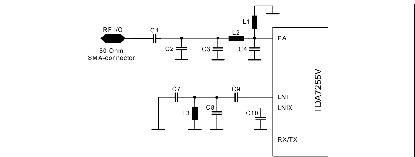
Figure 25 TX_Mode_Simplified
