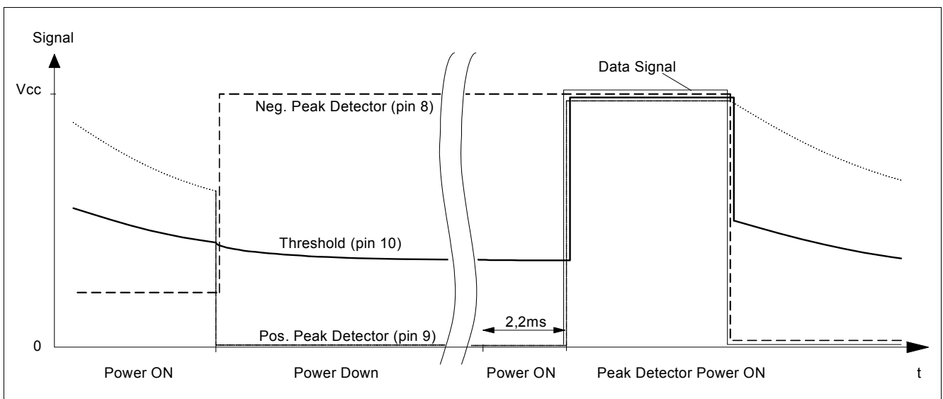
Figure 48 Power Down Mode
