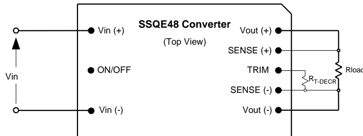
Figure D. Configuration for decreasing output voltage.
