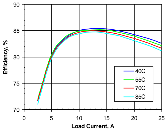
Figure 3. Efficiency vs. load current and ambient temperature for SSQE48T25012 converter mounted vertically with V_{in} = 48\text{ V} and air flowing from pin 1 to pin 3 at a rate of 200 LFM (1.0 m/s).
