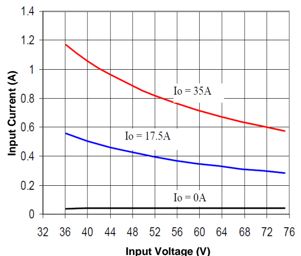
Figure 2. Input Characteristics ( 25^\circ\text{C} )
