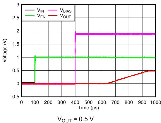
Figure 6-17. Startup With V_{BIAS} Powering Up After V_{IN} and V_{EN}
