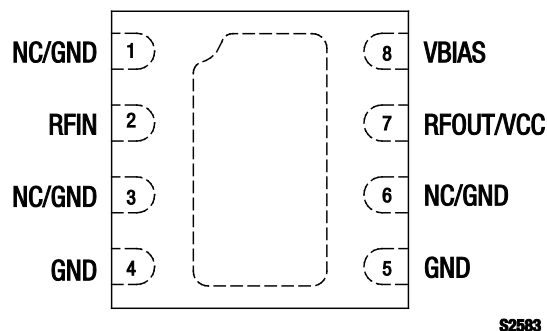
Figure 2. SKY67130-396LF Pinout – 8-Pin DFN (Top View)
