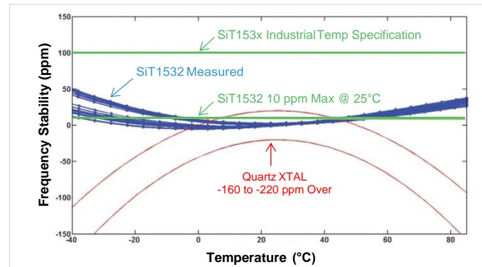
Figure 3. SiTime vs. Quartz
