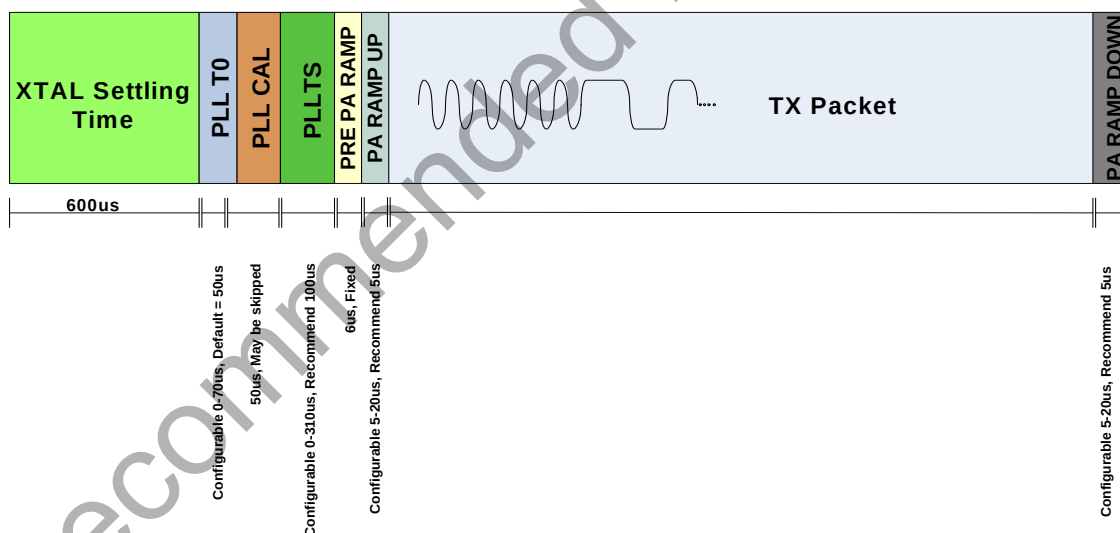
Figure 23.2. TX Timing
