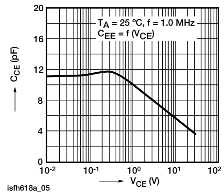
Fig. 7 - Transistor Capacitance
