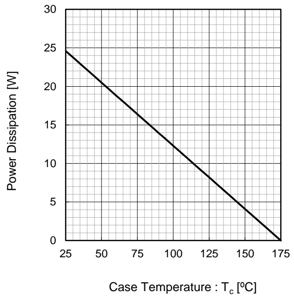
Fig.6 Power Dissipation
